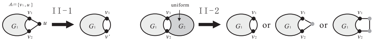
Figure 2: Reduction II based on 2-separation (G_1, G_2) at \{v_1, v_2\} .
