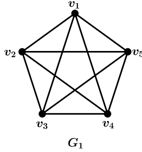
Figure 10: The primitive graph G_1
