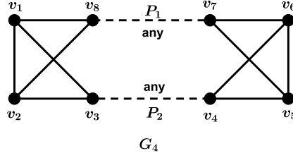
Figure 13: The primitive graph G_4
