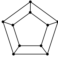
Figure 1: A graph G for which \pi(G) is not box-TDI
