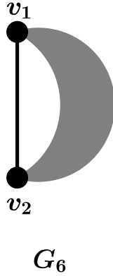
Figure 15: The primitive graph G_6
