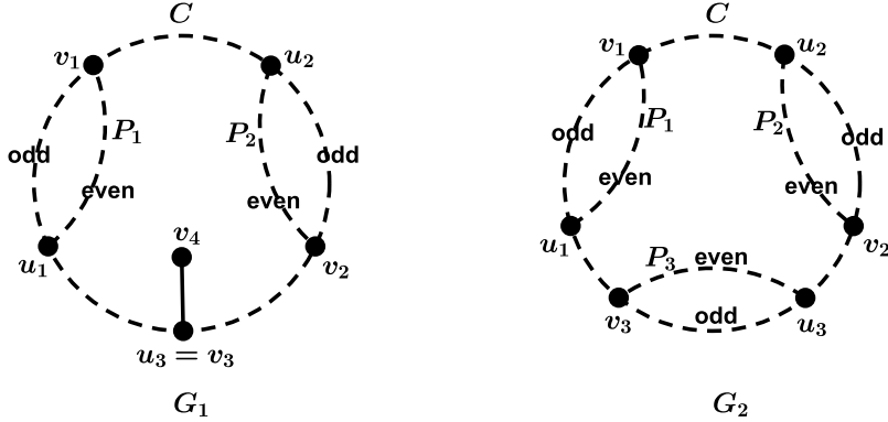
Figure 5: Two configurations with F_1 or F_2
