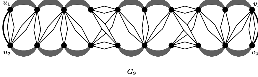
Figure 18: The primitive graph G_9
